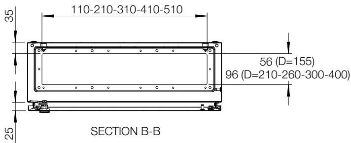
Sectional top view
