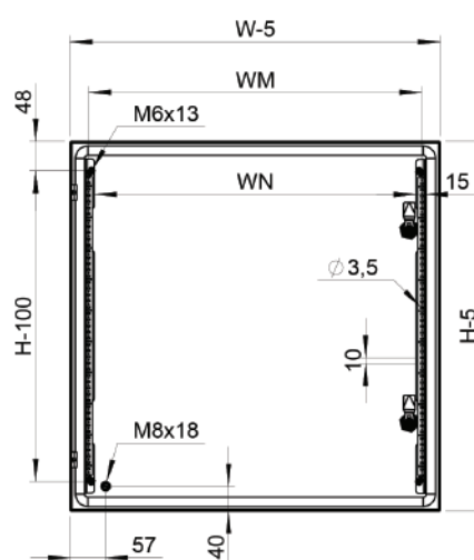
Inside door view
