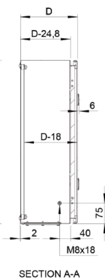
Sectional side view
