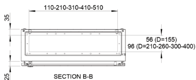
Sectional top view
