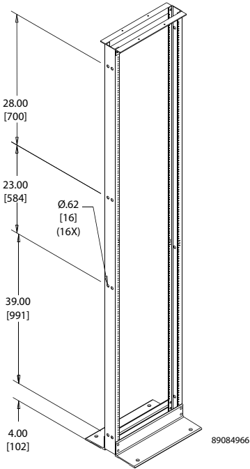
8-Foot and 9-Foot Racks Only (Width and Depth dimensions identical to 7-foot rack)
